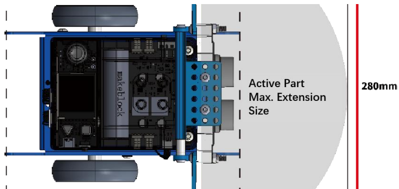
Figure 5.1-1 Maximum extension state (Side View)
